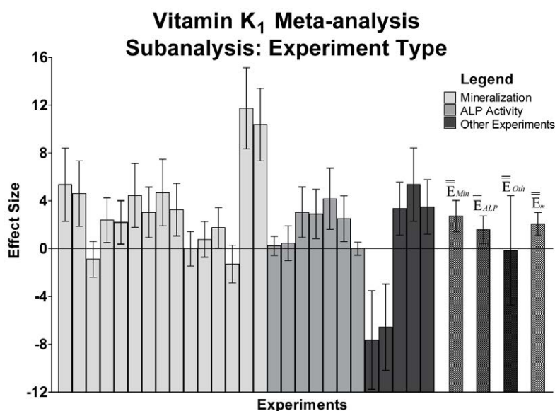
In the graph displaying the vitamin K 1 meta-analysis that was grouped by experiment type, each unlabelled bar represents the effect size of an experiment, as measured using the Hedges' d method. The bars were shaded according to experiment type and the error bars represent 95% confidence intervals. The grand means for each experiment type is signified by \bar{E} and a short form for each experiment name and the overall grand mean is signified by \bar{E}_m . The experiments used in the vitamin K 1 meta-analysis were extracted from 5 articles.
