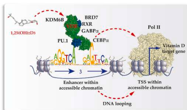
Fig. 4. Principles of vitamin D signaling. VDR is activated by 1,25(\text{OH})_2\text{D}_3 and interacts with a number of nuclear proteins, such as RXR, PU.1, CEBP \alpha , GABP \alpha , KDM6B and BRD7, and with genomic regions formed by DR3-type binding sites within enhancer regions. Activated VDR bridges via Mediator complex with Pol II binding to TSS regions of vitamin D target genes. In net effect, the expression of the target genes is up- or downregulated.
