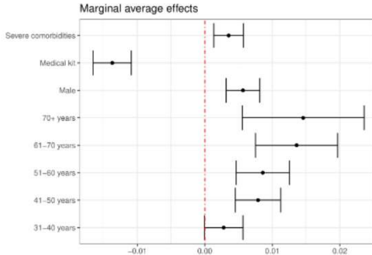
Figure 3: Marginal effects of ivermectin on hospitalization with administrative rule database. Subsets at between 80 y 85% of hospital occupancy (6).
