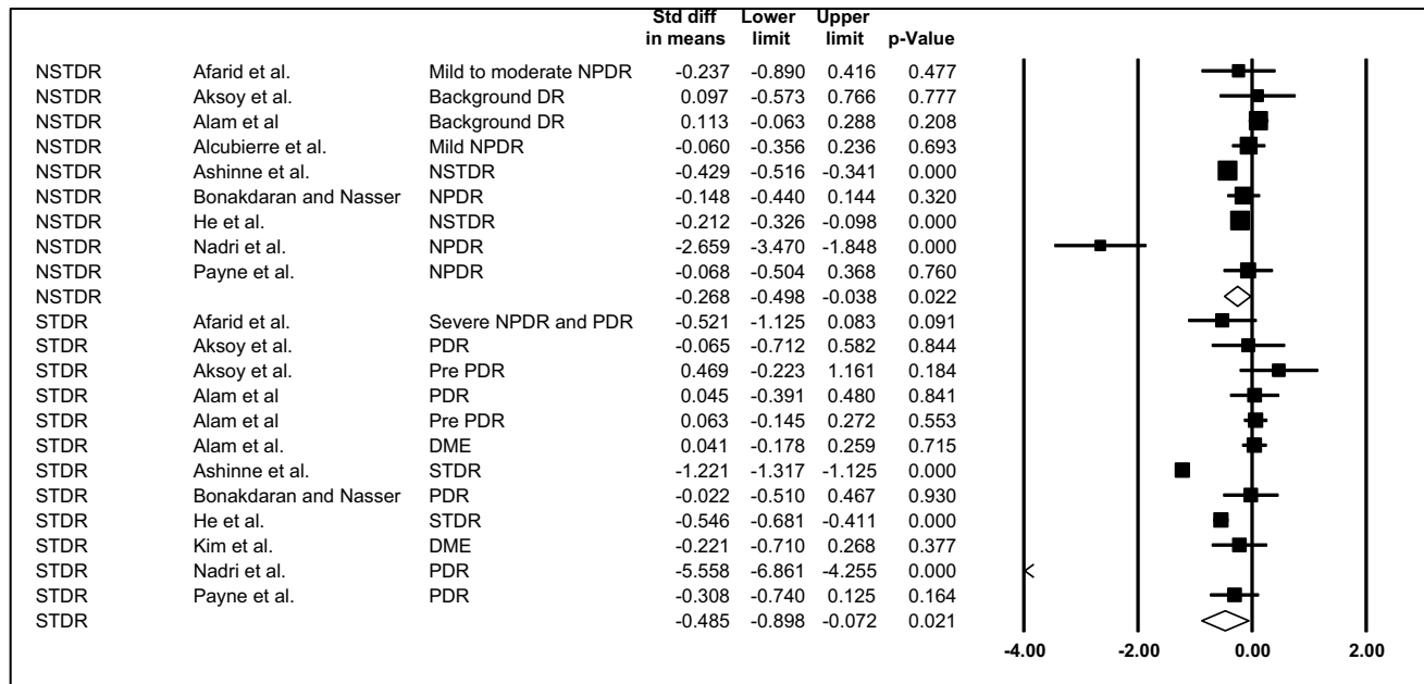
Fig. 3 Forest plot showing standard differences in means in 25(OH)D levels between people with versus without diabetic retinopathy
