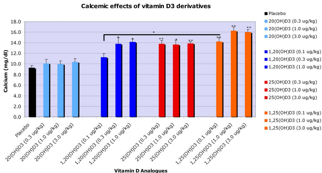
Figure 1. 20(OH)D 3 and 1,20(OH) 2 D 3 have less calcemic effect in comparison to 1,25(OH) 2 D 3 . In vivo testing of calcemic effects of 20(OH)D 3 and 1,20(OH) 2 D 3 in comparison to 1,25(OH) 2 D 3 . doi:10.1371/journal.pone.0009907.g001
