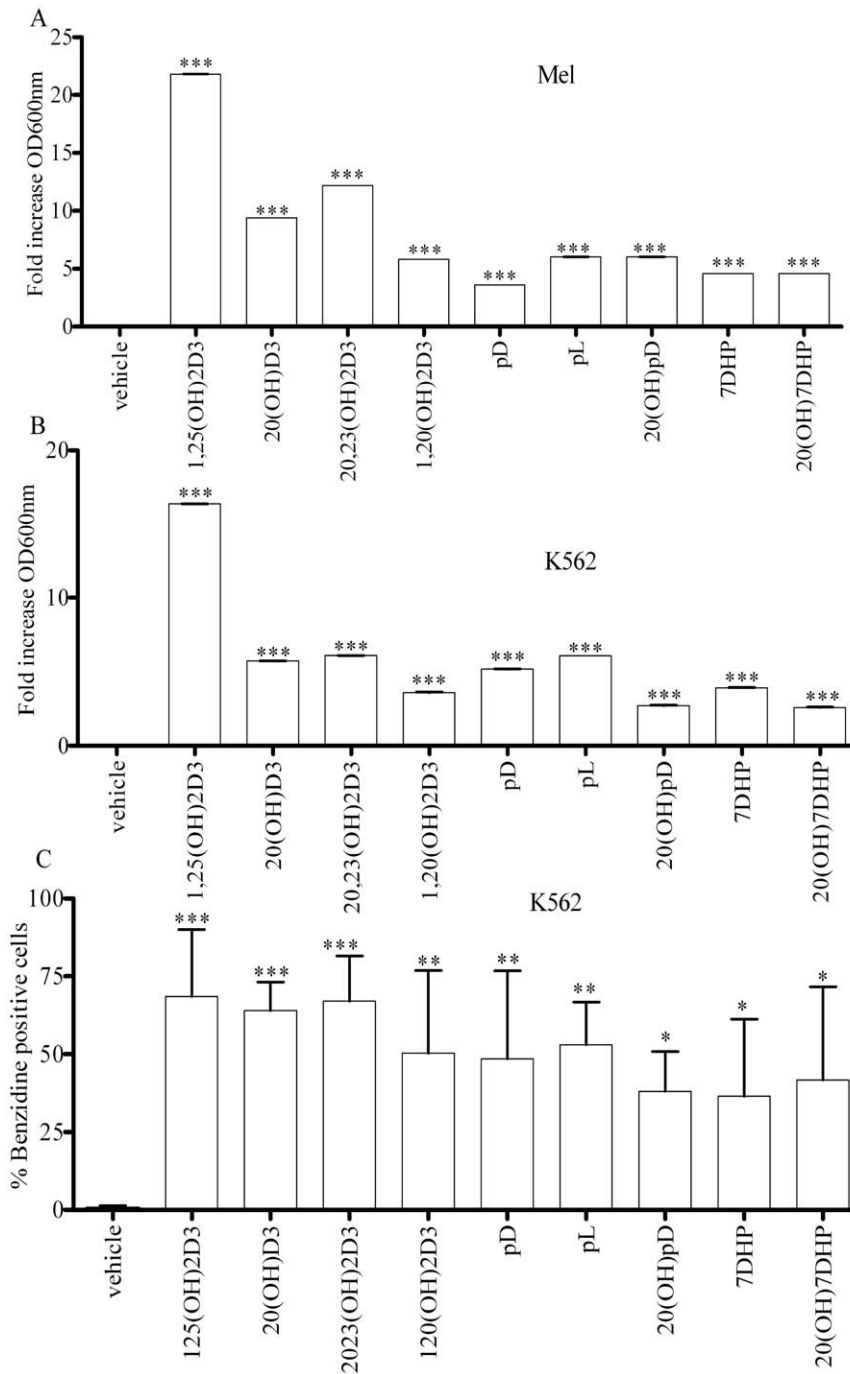
Figure 3. Novel secosteroids and steroidal 5.7-diene induce erythroid differentiation in leukemia cells. Induction of erythroid differentiation determined was from the the concentration of hemoglobin in an equal number of cells. Cells were treated for 7 days with different compounds ( 10^{-7} M), stained with benzidine solution and the amount of hemoglobin as hemin in Mel (A) or K562 (B) leukemia cells was determined by measuring the absorbance at 600 nm after lysis of the cells. *** p < 0.001 . C. The number of benzidine positive K562 cells after 7 days of treatment with different compounds ( 10^{-7} M). Cells were stained with benzidine solution and the number of benzidine positive (blue) cells was determined by counting 200 cells per microscopic field. The results are present as % of benzidine positive cells in comparison to total cell number. * p < 0.05 ; ** p < 0.01 ; *** p < 0.001 . doi:10.1371/journal.pone.0009907.g003
