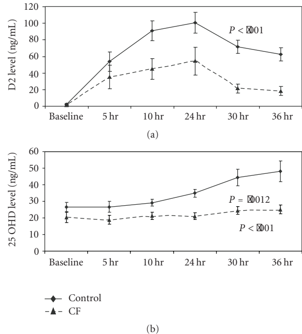
FIGURE 2: Impaired absorption of Vitamin D following a 2500 µg dose in CF patients and controls [13].
