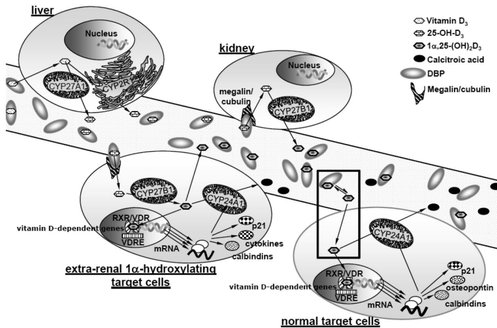
FIGURE 1. Free 1,25-dihydroxyvitamin D theory of target cell entry. This figure depicts most components of vitamin D signal transduction. Vitamin D 3 (upper left side of the diagram) is carried to the liver, where one of a series of 25-hydroxylases—the major ones are the microsomal CYP2R1 and the mitochondrial CYP27A1—activates it. The resulting 25-hydroxyvitamin D 3 [25(OH)D 3 ] is then carried on vitamin D binding protein (DBP) to the kidney, where the classic renal CYP27B1 1 \alpha -hydroxylates it and puts it back into circulation as 1 \alpha ,25-dihydroxyvitamin D 3 [1 \alpha ,25(OH) 2 D 3 ]. 1 \alpha ,25(OH) 2 D 3 then enters and acts on vitamin D target cells at the level of gene transcription through a VDR-mediated mechanism (cell at bottom right). Note that according to this vitamin D signal transduction, 1 \alpha ,25(OH) 2 D 3 arrives at the target cell bound to DBP, but its entry into the cell is a function of the free pool of 1 \alpha ,25(OH) 2 D 3 (shown inside the red box) in equilibrium with protein-bound 1 \alpha ,25(OH) 2 D 3 . In hypervitaminosis D, some investigators argue that saturation of the DBP displaces a greater amount of free 1 \alpha ,25(OH) 2 D 3 , thereby increasing gene expression and causing hypercalcemia and other toxicity symptoms. According to the extrarenal 1 \alpha -hydroxylase theory, some target cells express the membrane proteins megalin or cubulin to concentrate the 25(OH)D 3 -DBP complex and express the protein CYP27B1 to 1 \alpha -hydroxylate 25(OH)D. Some believe that in this way, certain target cells (eg, macrophages and monocytes) boost 1 \alpha ,25(OH) 2 D 3 production by augmenting the circulating 1 \alpha ,25(OH) 2 D 3 concentrations produced by the kidney. Although research has not proven the theory, many of its facets are consistent with the observed health advantages of vitamin D and with emerging epidemiologic data (2, 3). Adapted with permission from reference 4. RXR, retinoid X receptor; VDR, vitamin D receptor; VDRE, vitamin D responsive element.
